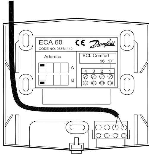
Danfoss 87B281.11
