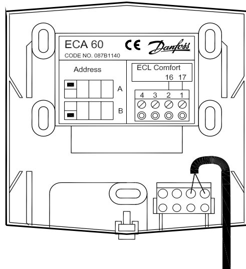
Danfoss 87B283.11
